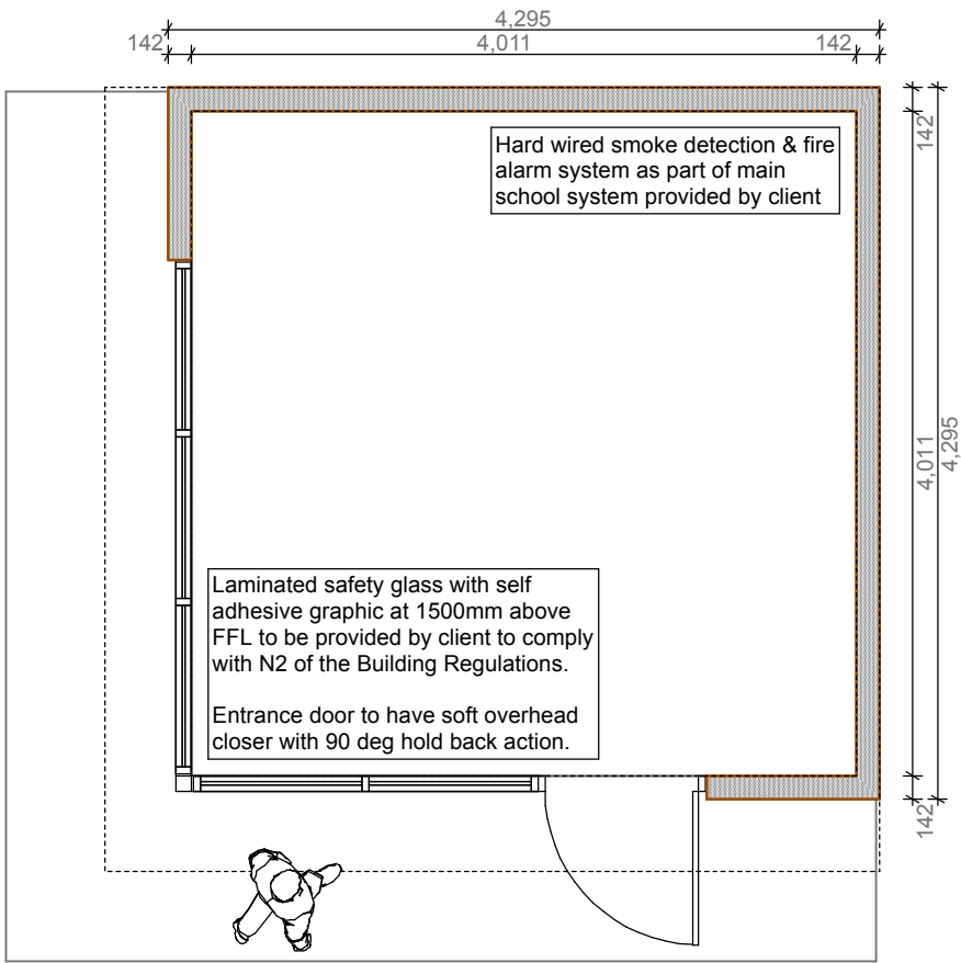
Floor Plan 1:50
