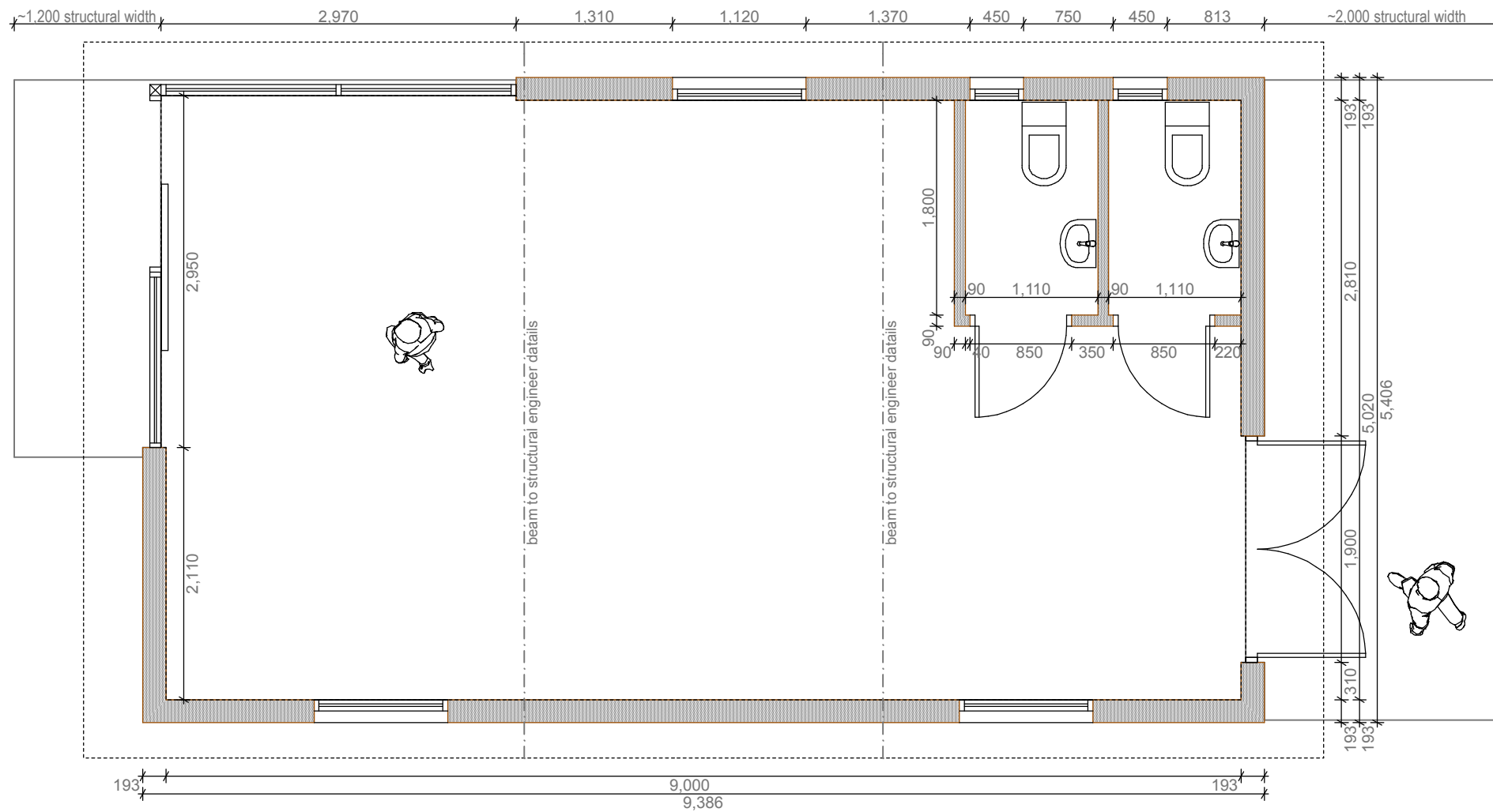
Plan Layout 1:50
