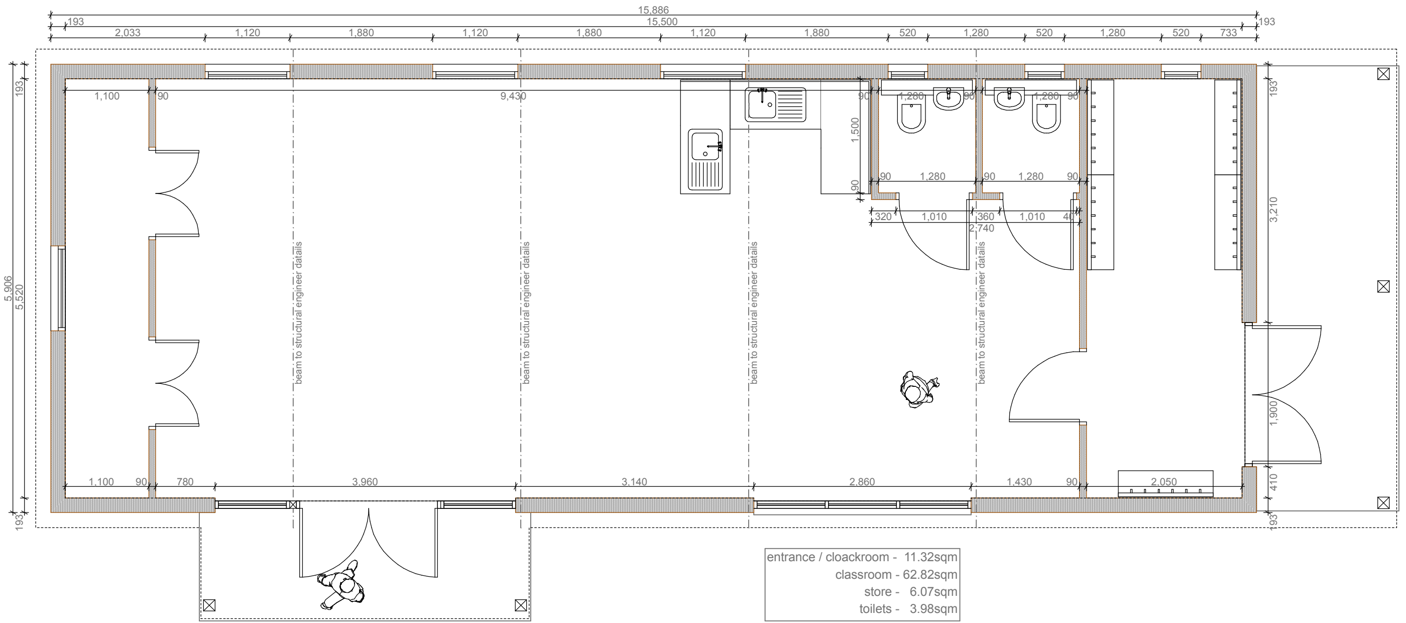
Plan Layout 1:50
