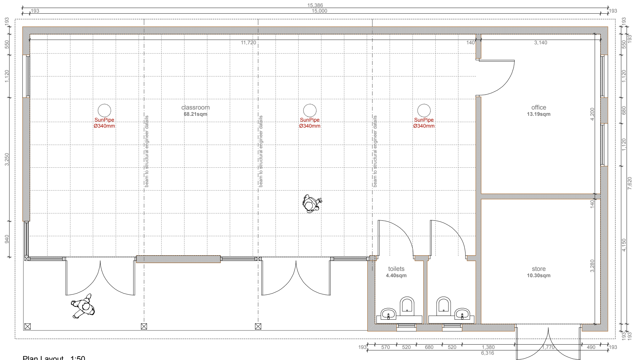
Plan Layout 1:50
