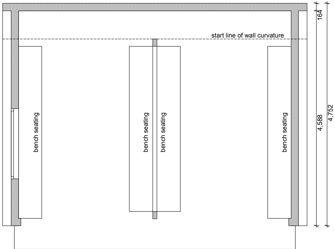
Floor Plan 1:50
