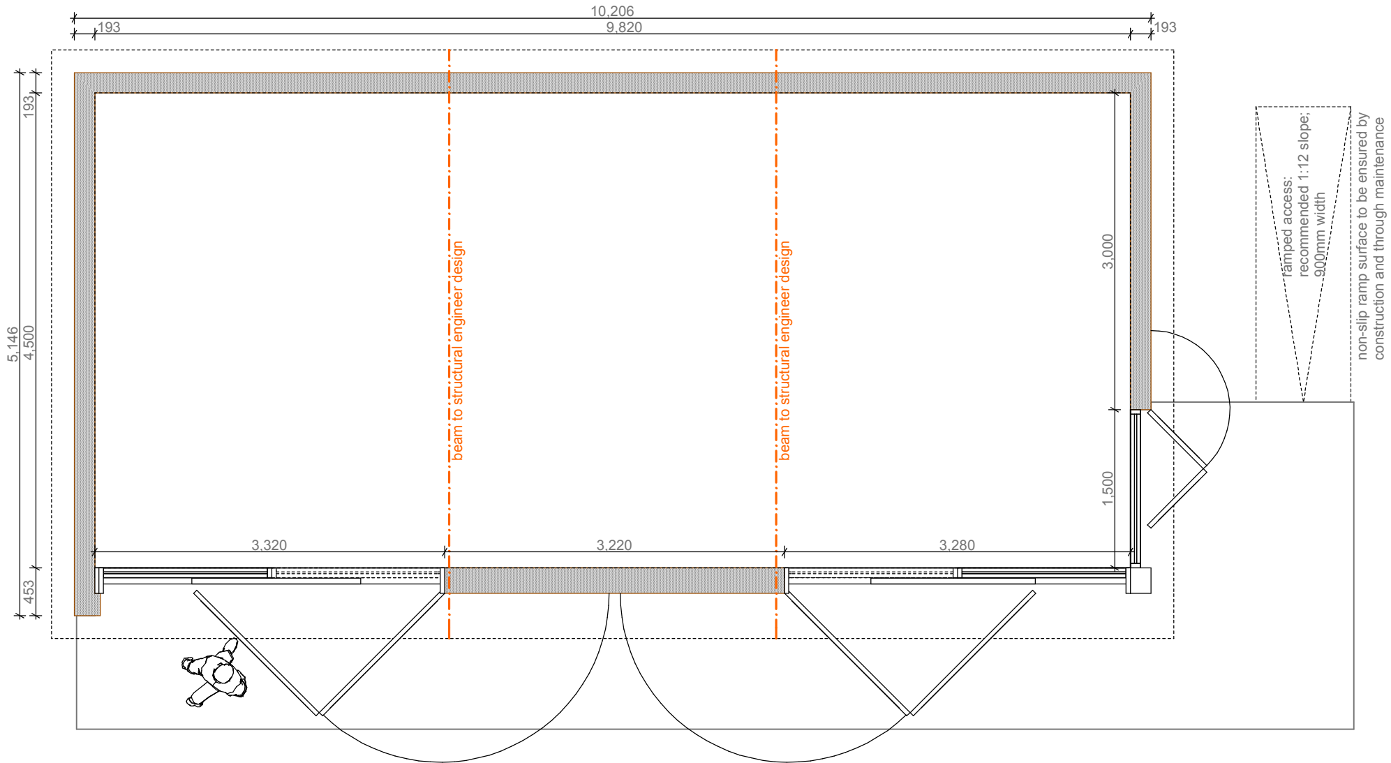
Plan Layout 1:50
