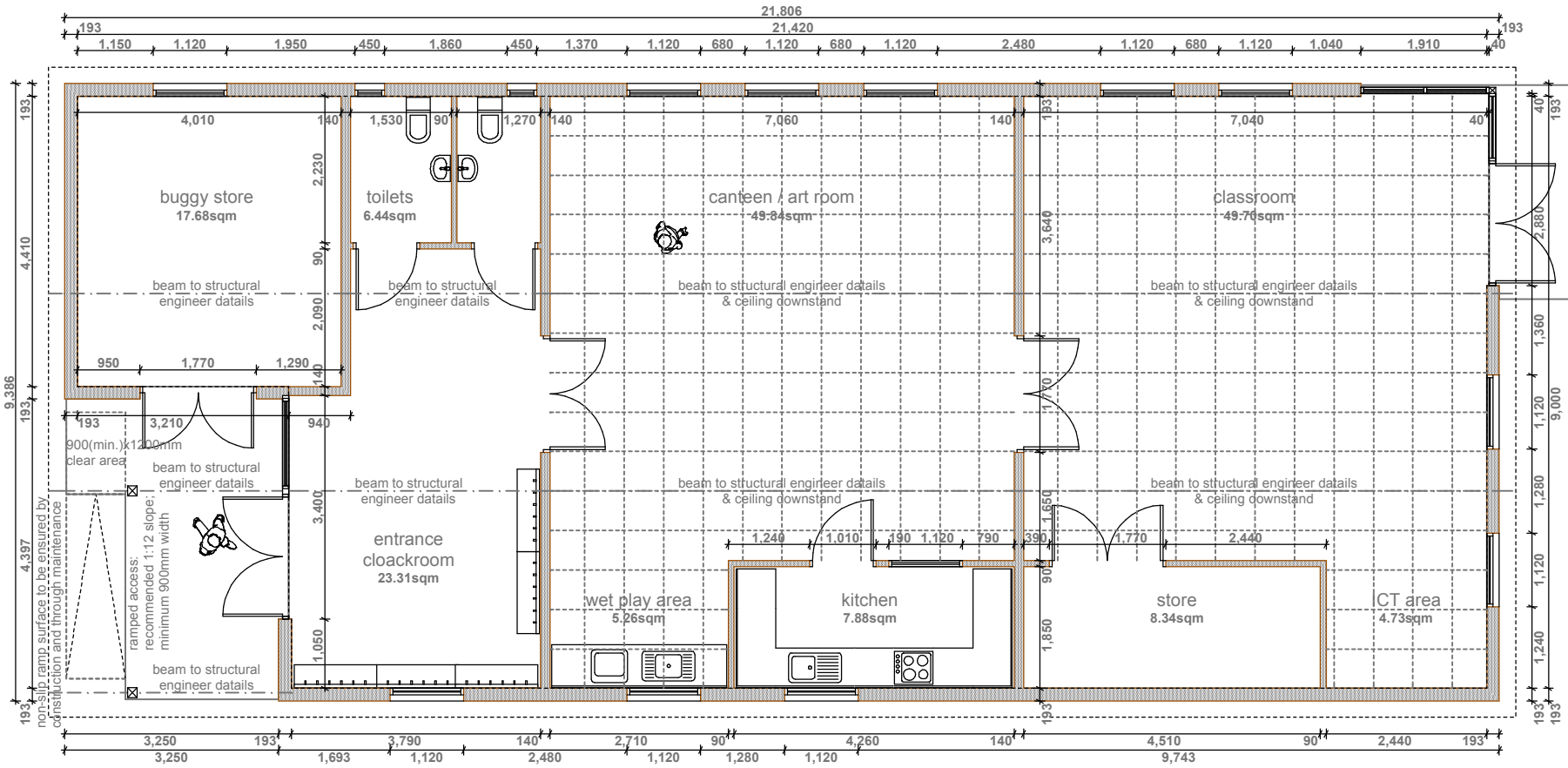
Plan Layout 1:100
