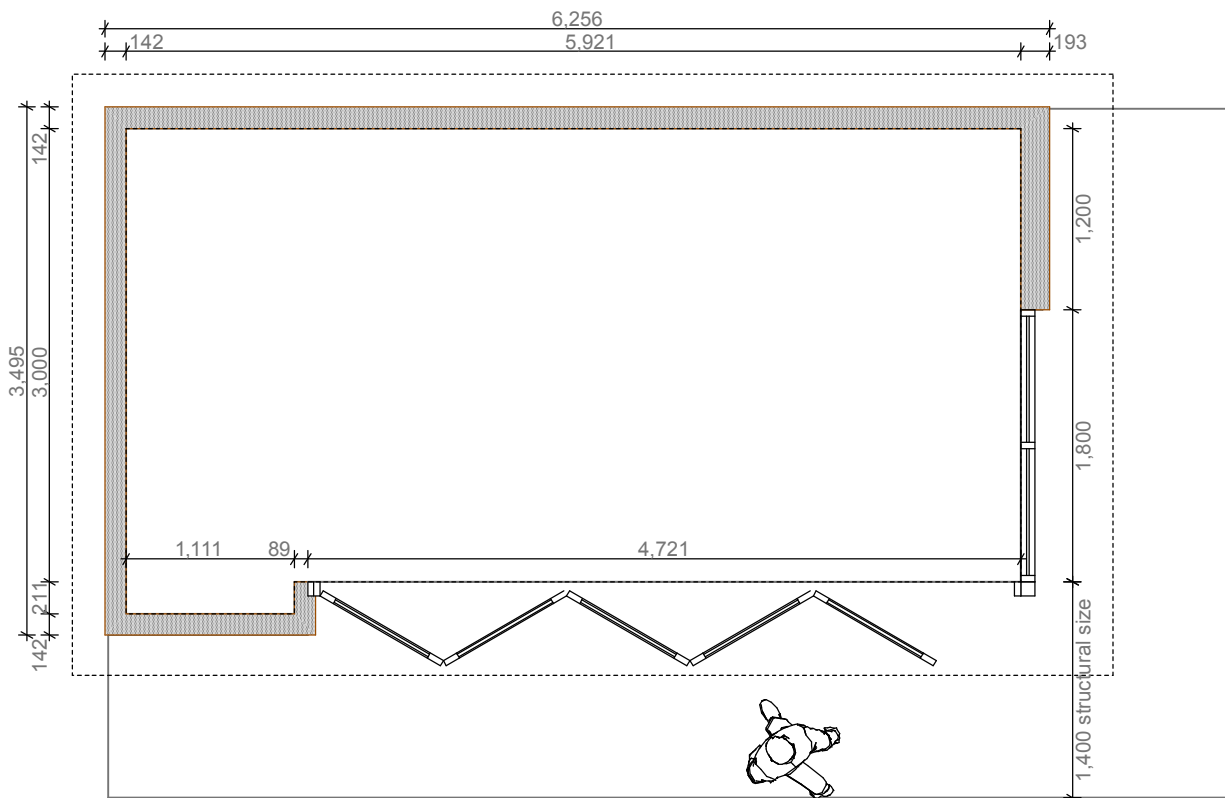
Floor Plan 1:50
