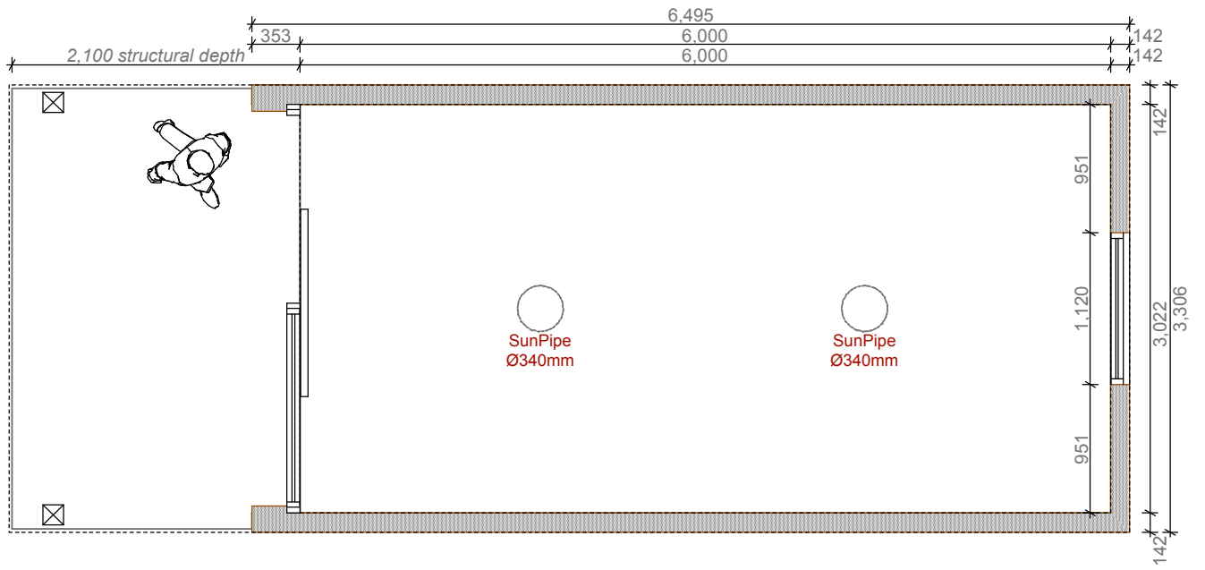
Floor Plan 1:50
