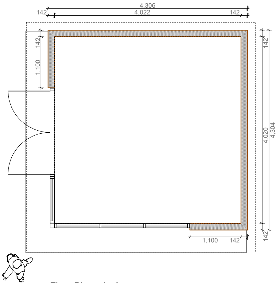
Floor Plan 1:50
