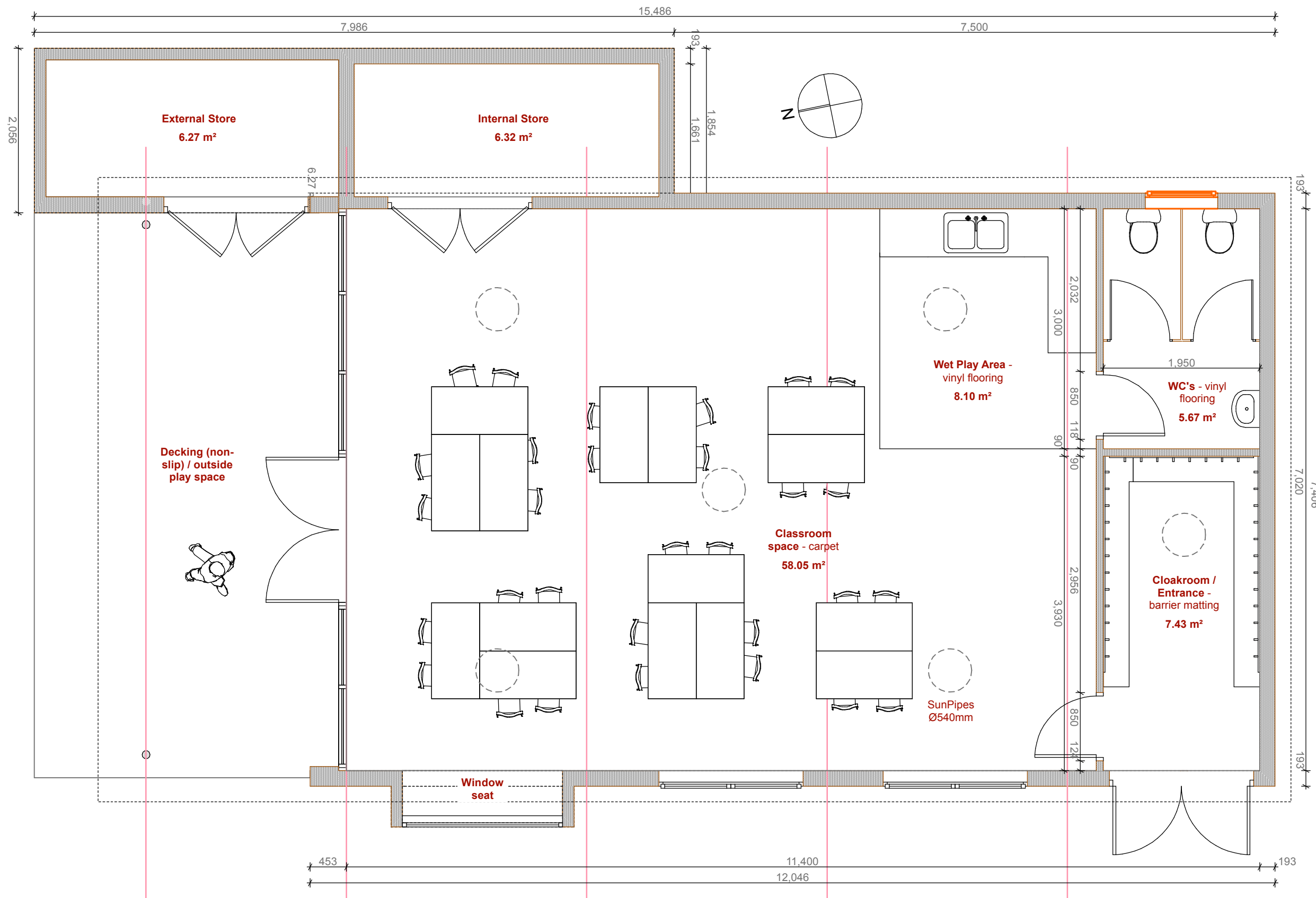
Floor Plan - 1:50
